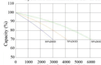
Cycle life in relation to DOD at 25°C
