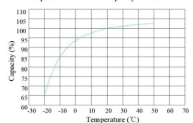
Temperature effects on capacity at 0.2C
